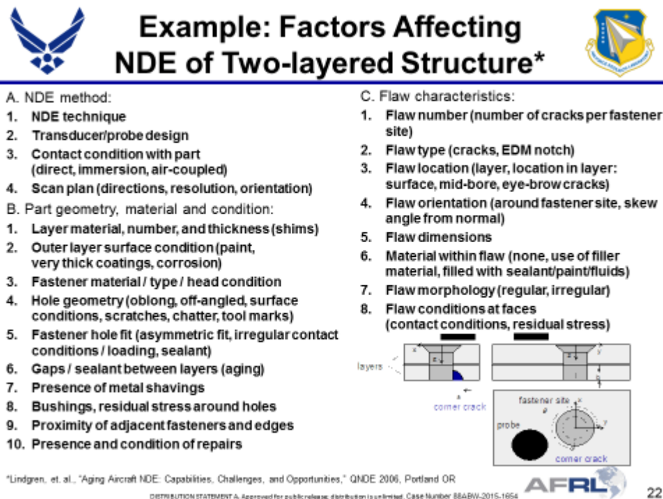
Figure 2. List of twenty-two factors that can affect the ability to use ultrasound to detect a fatigue crack in a representative two-layer aircraft joint [11].
